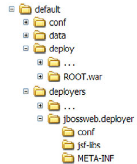
Figure 5.2 The main directories used to configure JBoss Web Server and to deploy web applications
